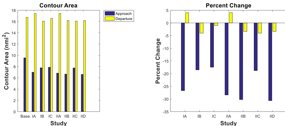
Figure 16. Aircraft-specific impact for studies I & II. 300 PAX
