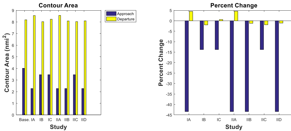
Figure 28. 100 PAX Studies I & II
