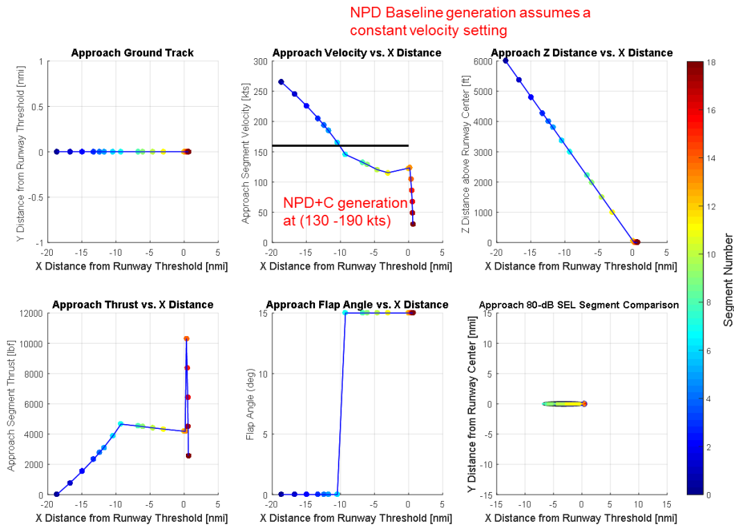
Figure 4. Vehicle specific analysis 100 PAX, I.A - 1
