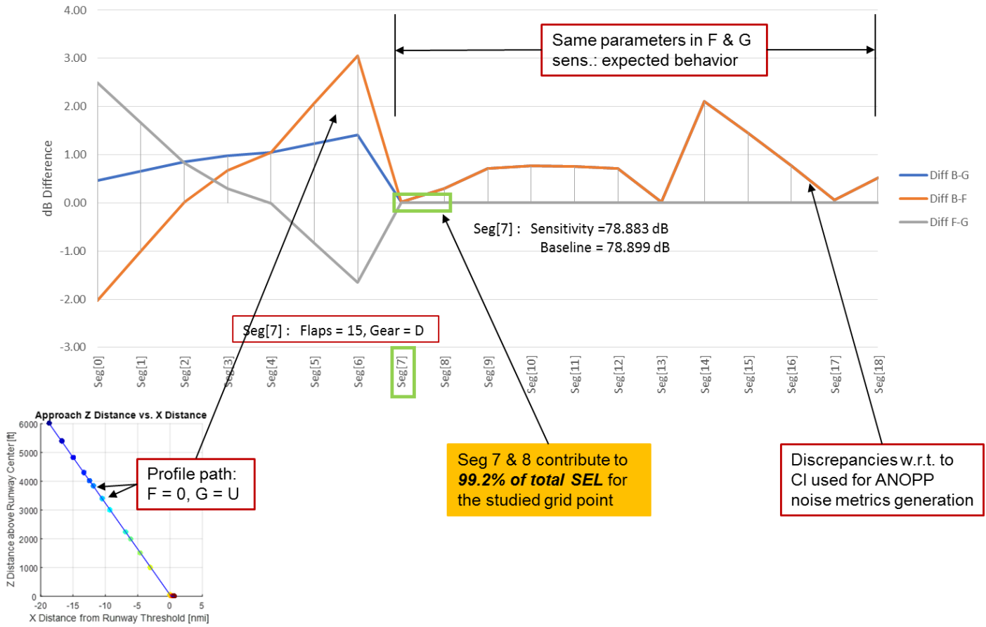
Figure 29. Segment-wise contribution - APPROACH 150 PAX
