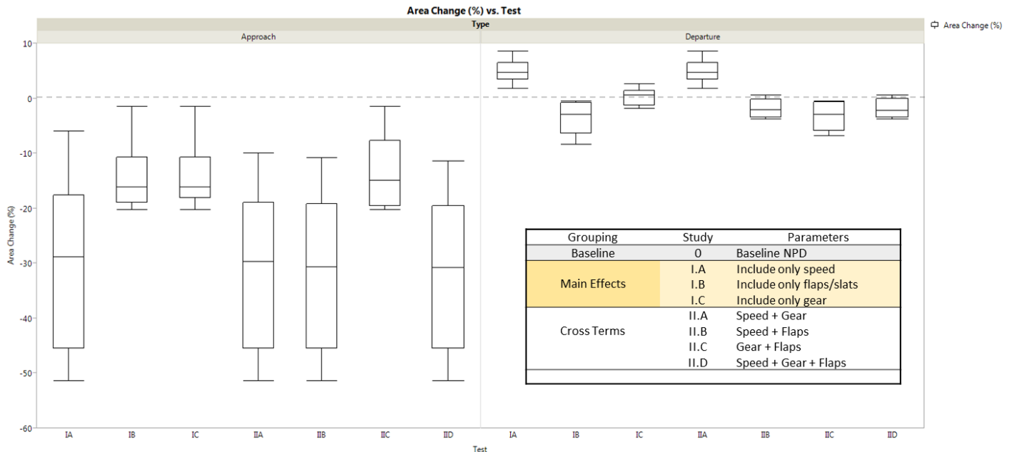
Figure 24. Noise contour area change (%) for all of the studies
