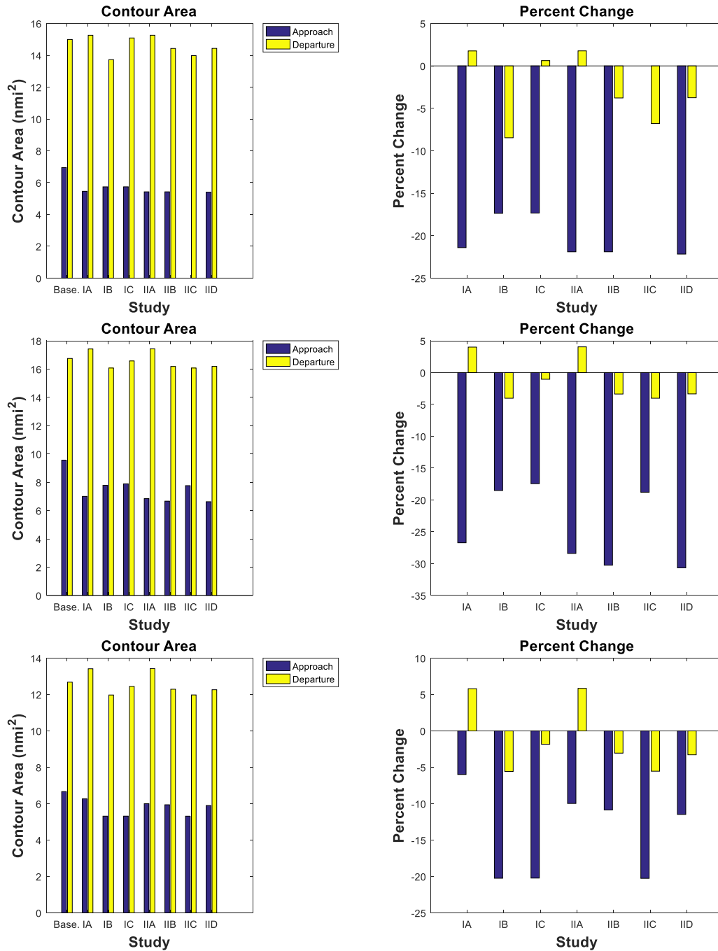
Figure 26. 210 - 300 - 400 PAX. Study I & II
