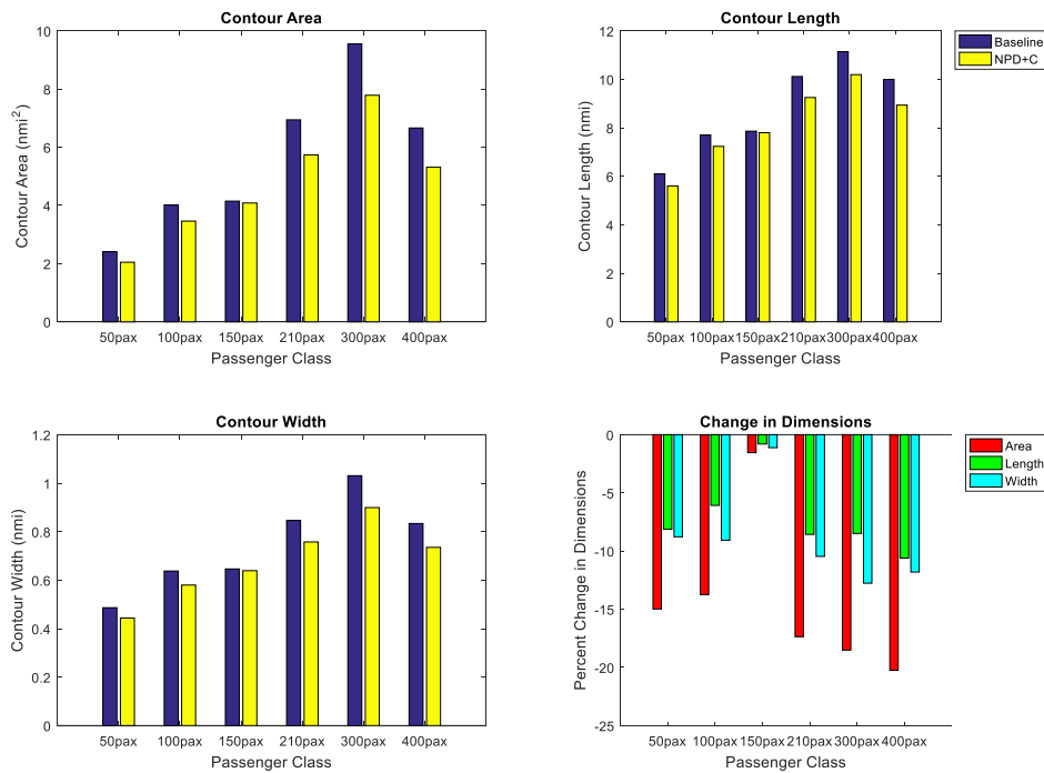
Figure 14. Study I.C Approach
