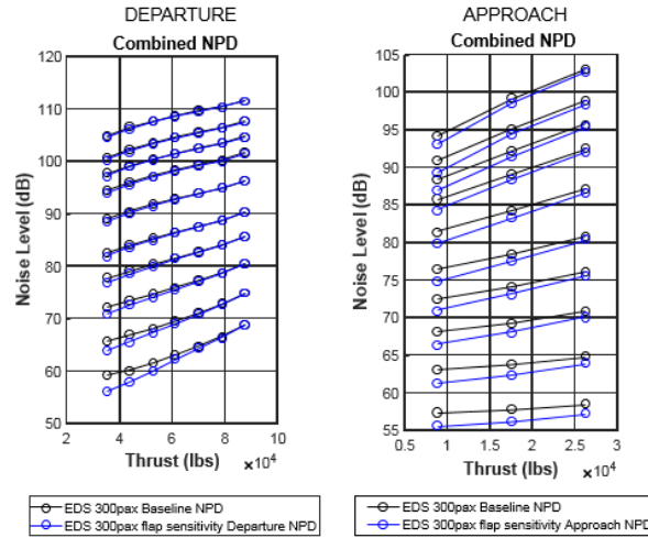
Figure 13. NPD vs. NPD+C most contributing segment. I.B
