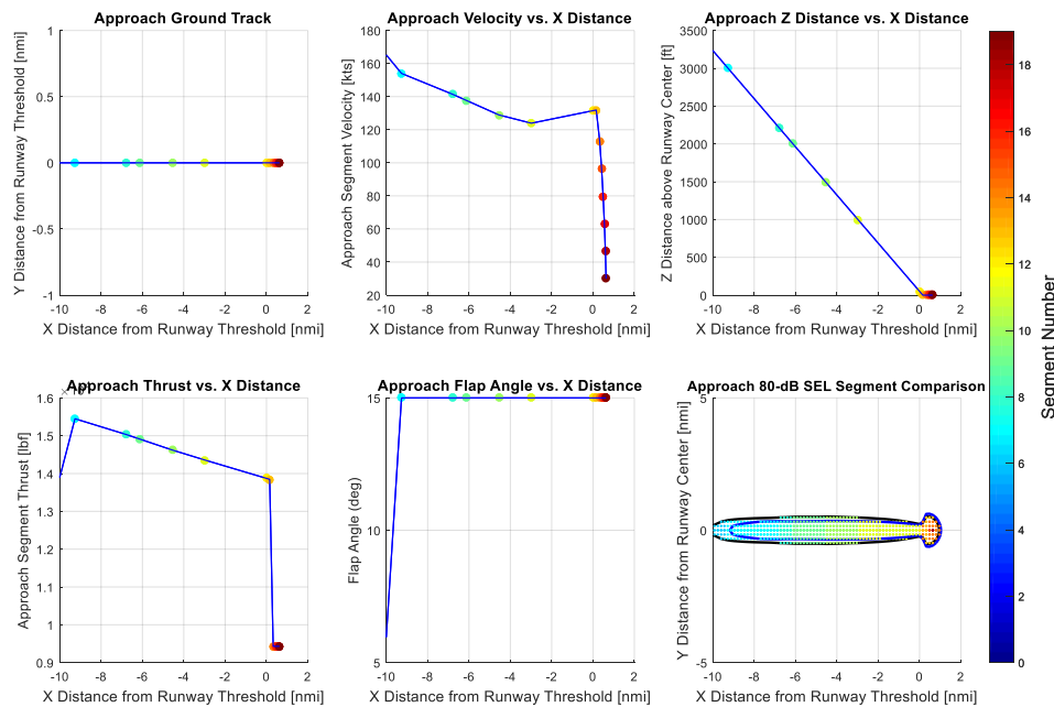
Figure 17. 300 PAX Study II.D - 1
