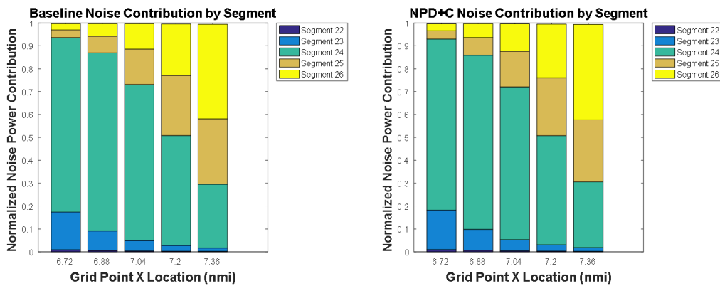
Figure 9. Analysis and noise contribution - 100 PAX I.A Departure
