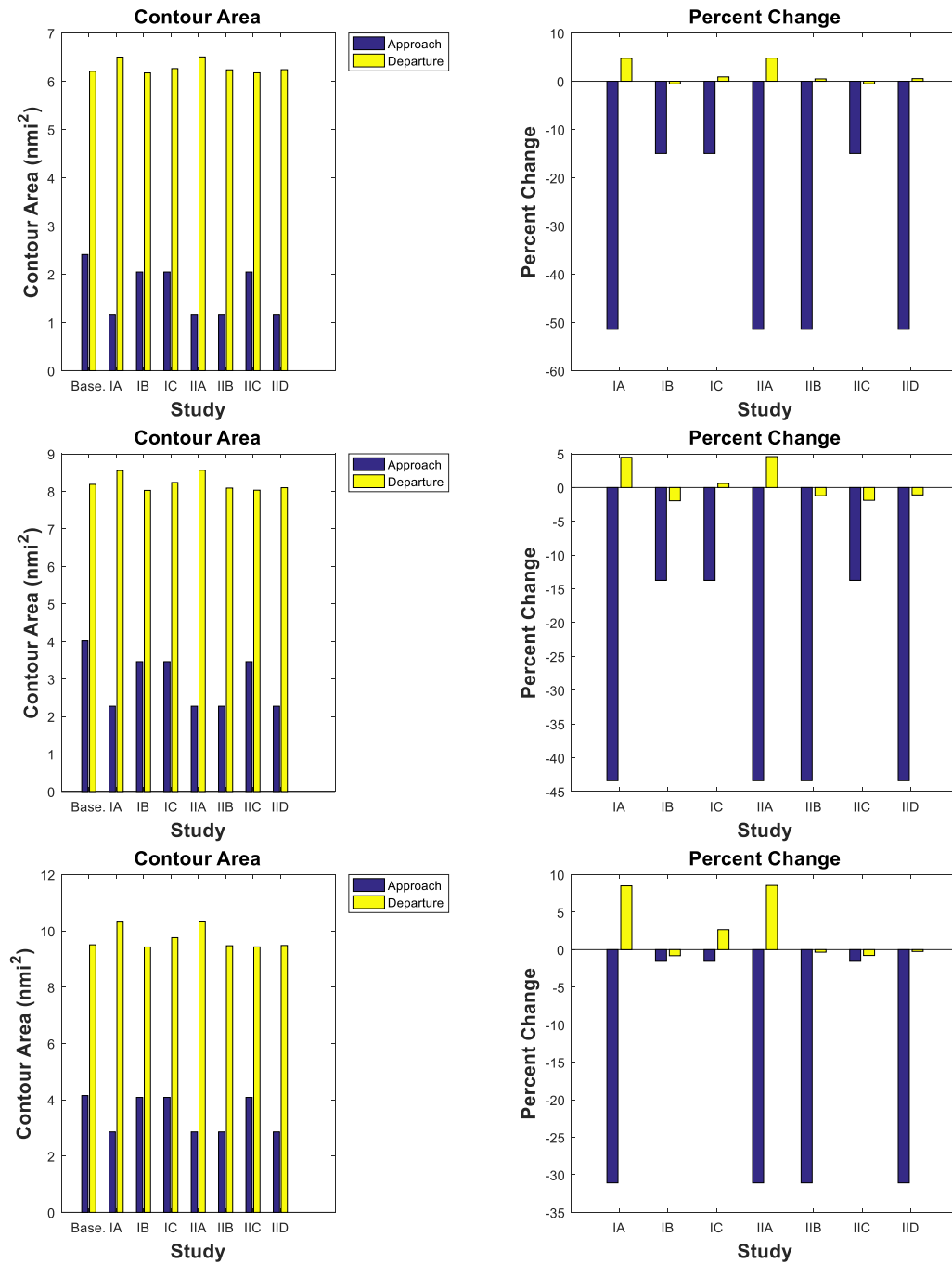
Figure 25. 50 - 100 - 150 PAX. Study I & II
