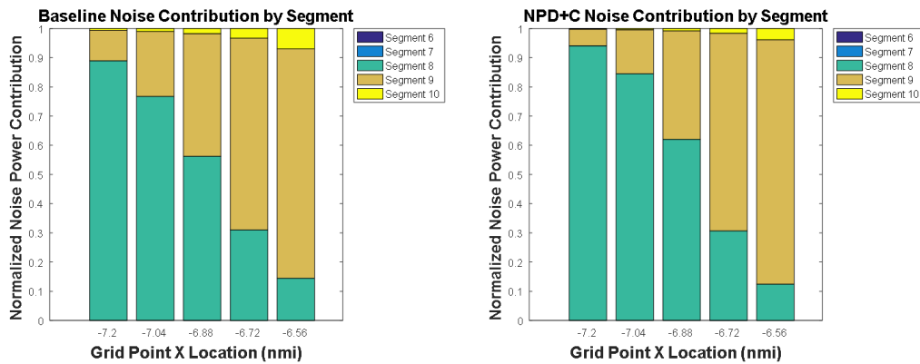
Figure 6. Vehicle Specific Analysis 100 PAX, I.A - 3
