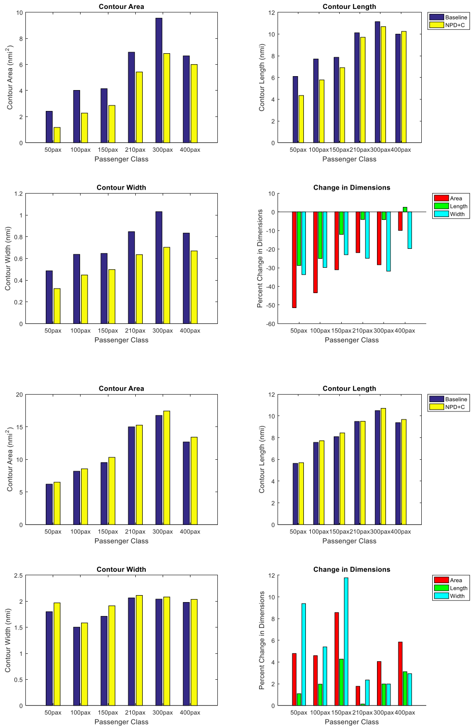
Figure 20. Study II.A Approach (top) - Departure (bottom)
