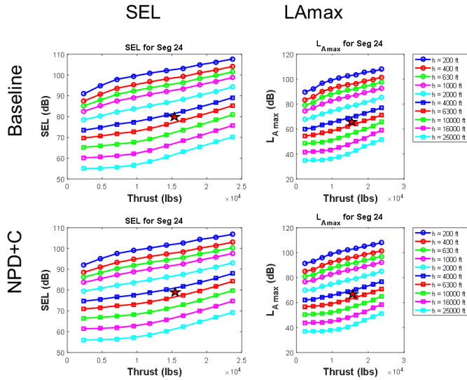
Figure 8. Segment NPD+C vs. NPD data
