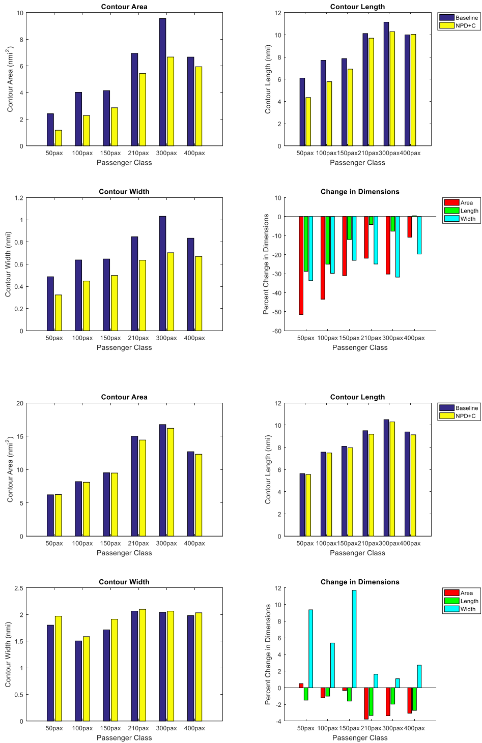
Figure 21. Study II.B Approach (top) - Departure (bottom)
