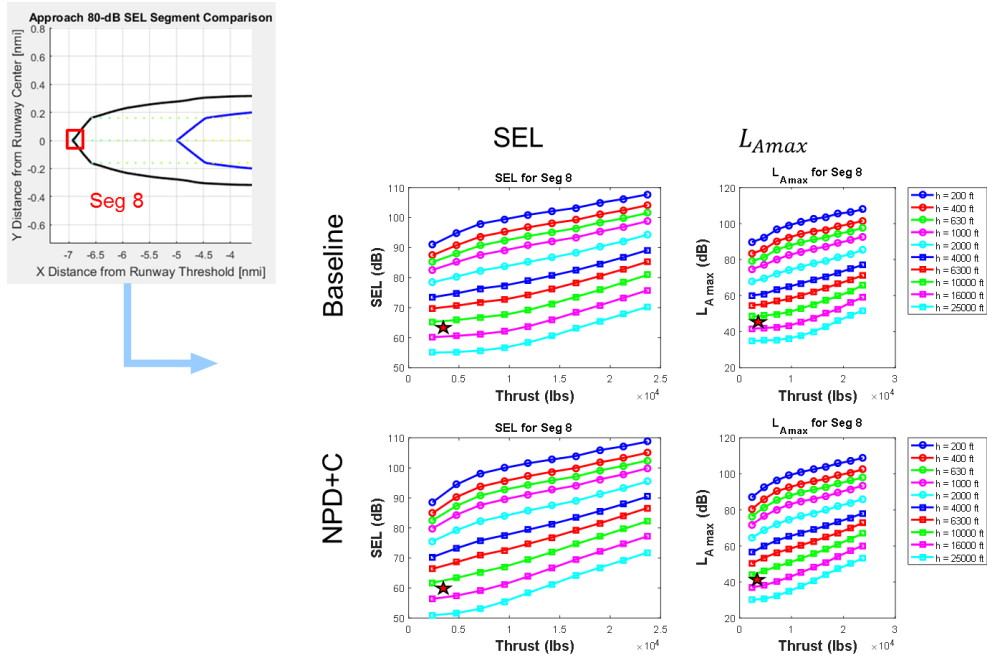
Figure 5. Vehicle specific analysis 100 PAX, I.A -2
