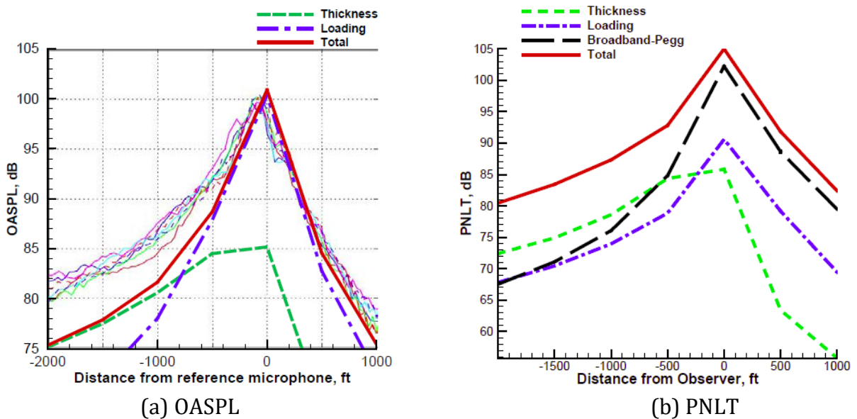
Figure 2.1 OASPL and PNLT levels for 80 kts level flight “housekeeping” run.
